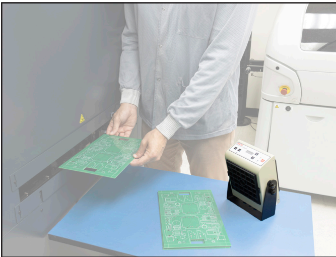
Figure 4. Using the 770122 Benchtop AC Ionizer at a machine station
