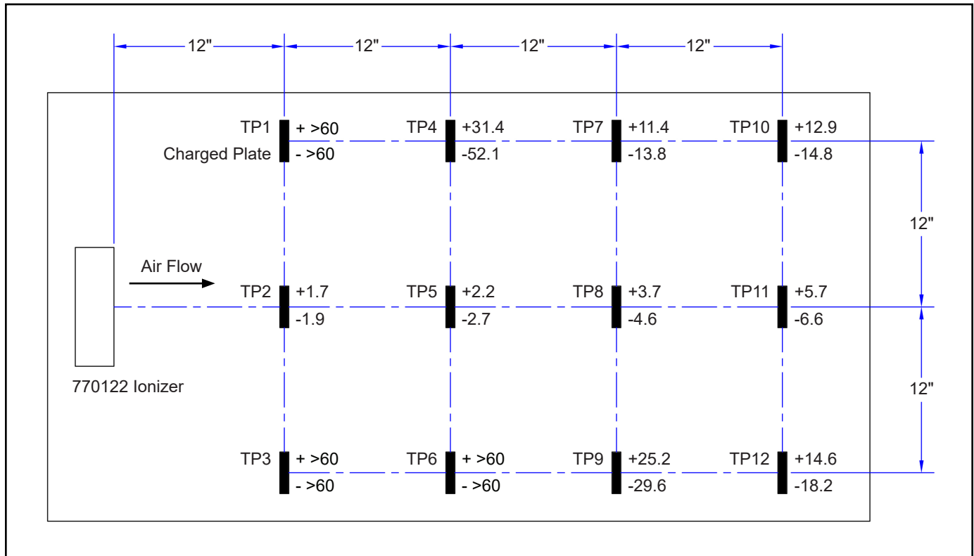
Figure 5. Neutralization (discharge) times in seconds at high fan speed
