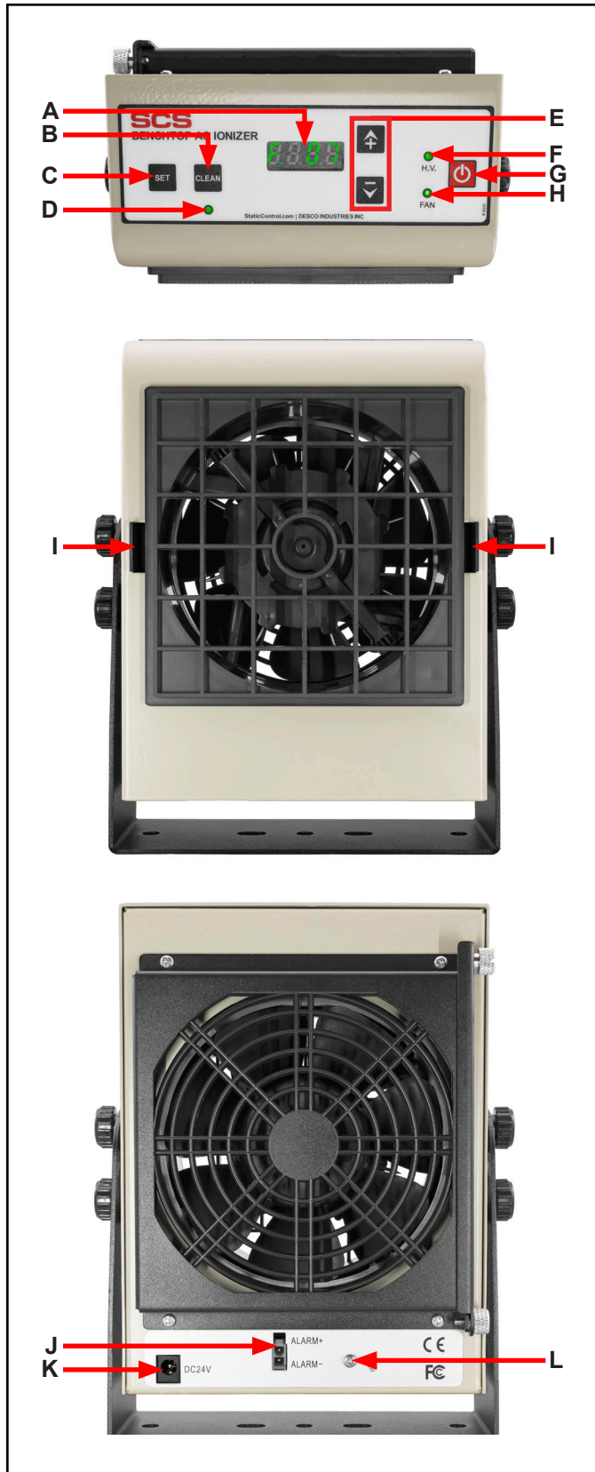
Figure 2. 770122 Benchtop AC Ionizer features and components
